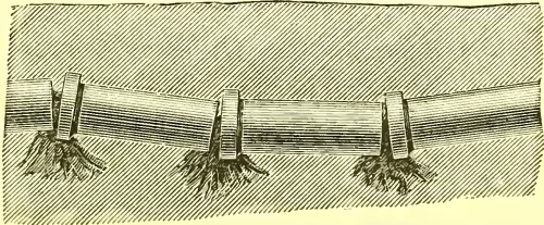
FIG. 1.—Drain in made land, settled. ("Sanitary Engineer.")
